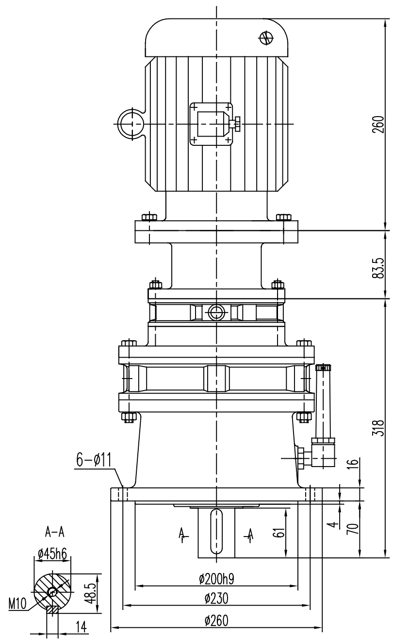
BLD20-1.1kw NER GROUP CO.,LIMITED 立式双级电机接盘型摆线针轮减速机 www.sogears.com
