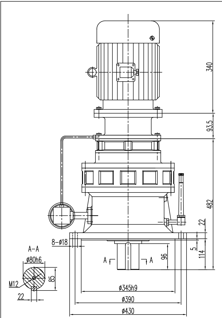
NER GROUP CO.,LIMITED XLED74-4kw www.sogears.com 立式双级电机接盘型摆线针轮减速机
